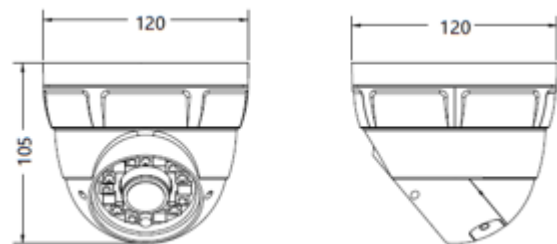
Figure 2-3 Dimensions (Unit:mm)
