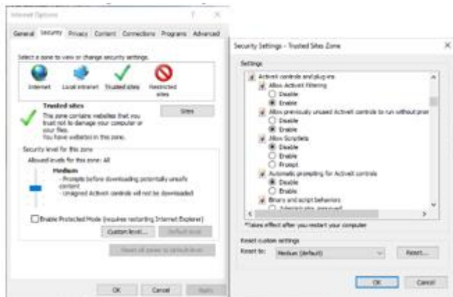
Figure 4-4 Configuring ActiveX Control and Plug-in
