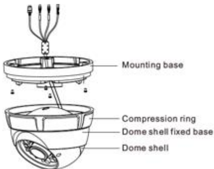
Figure 3-3 Camera Installation
