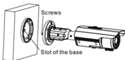
Figure 3-1 Installing Camera
