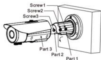
Figure 3-3 Loosening Screws
