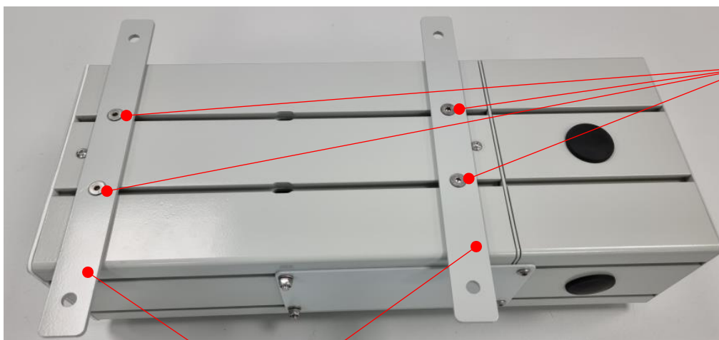
2 x Hub Wall Brackets
