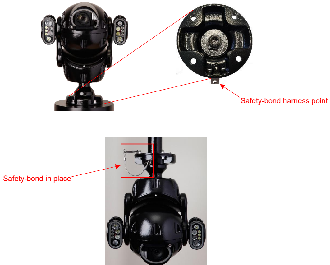
Fig. A PCD Direct-Mounting base (X2 COMBAT shown as example):
